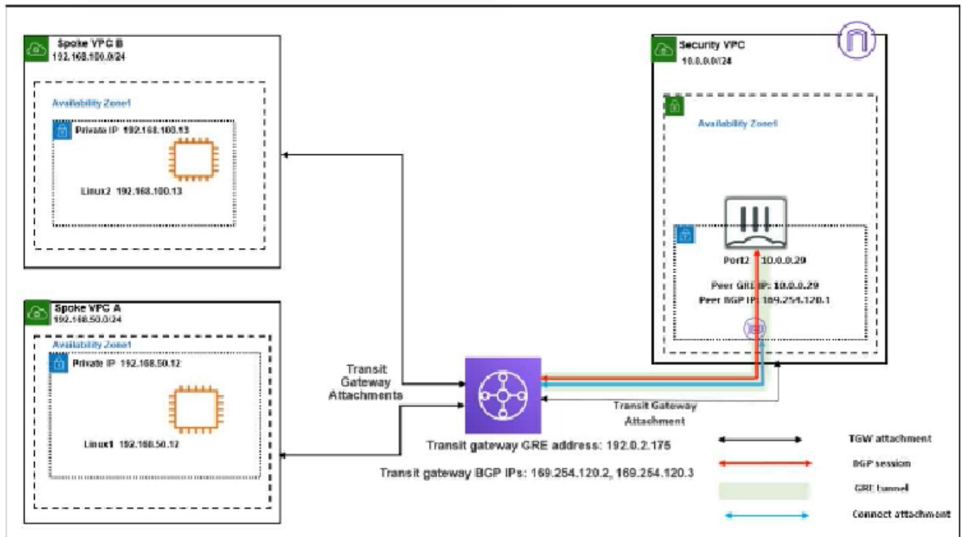
Network Topology
